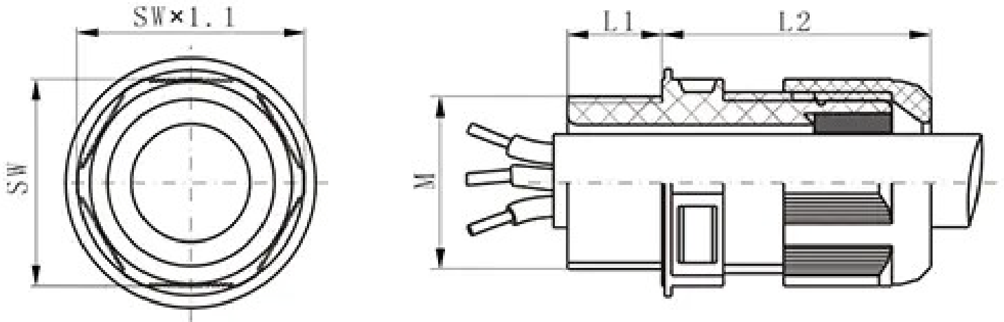
CZ0220/1 □ Plastic cable glands
