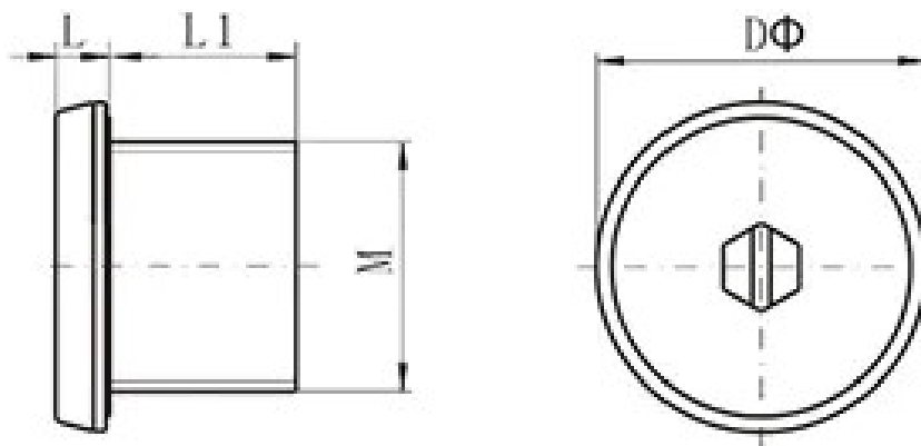
CZ0220/32 Plastic stopping plugs
