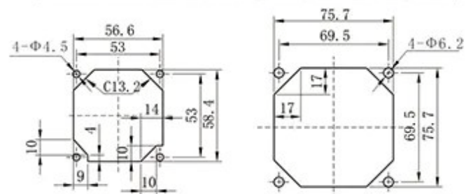
Installation dimensions of panel type socket
