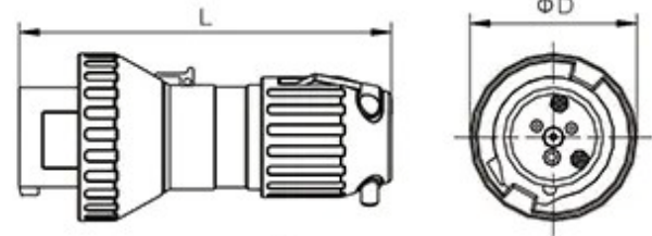
Plug
