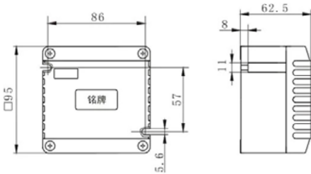
Size 1 CZ0520/□-21
