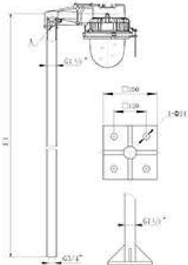
C — Lamp cap reserved in the angle of 90° Fanon type
