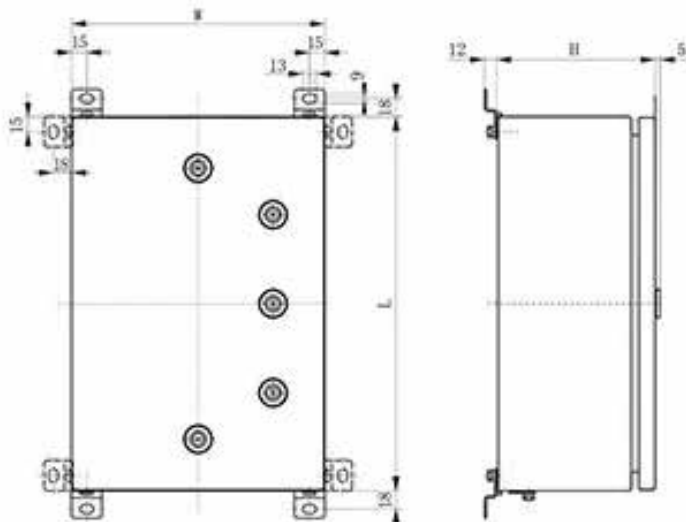
CZ1320 Stainless steel terminal box ( Door-open type )
