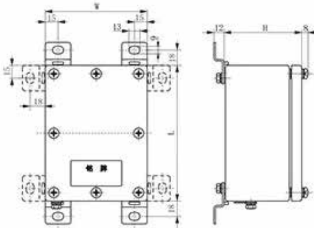
CZ1320 Stainless steel terminal box ( Cover-open type )
