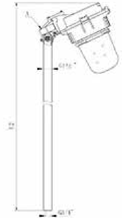
D — Lamp cap mounted in the angle of 23° (Inco type)
