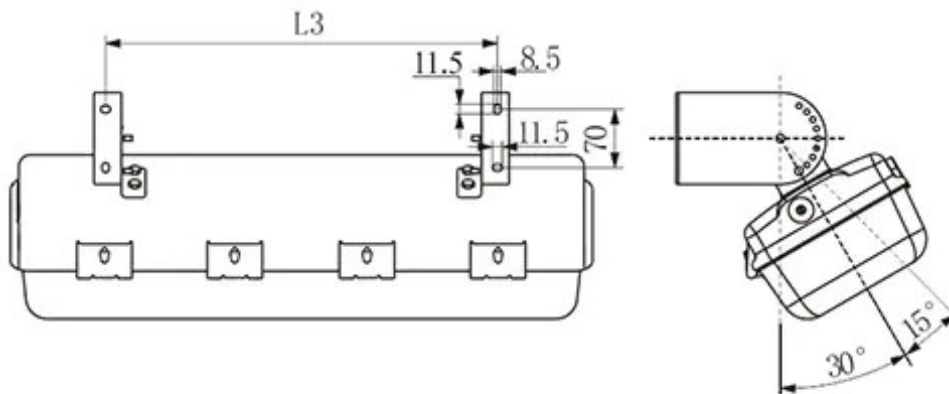
Adjustable mounting bracket
