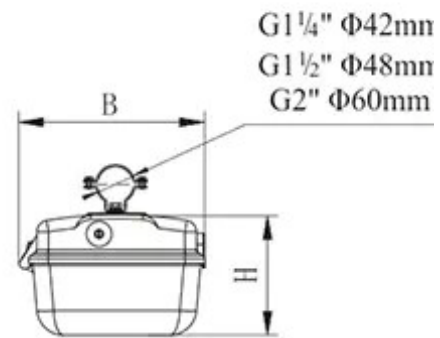
Clamp type
