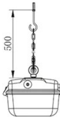
Chain type
