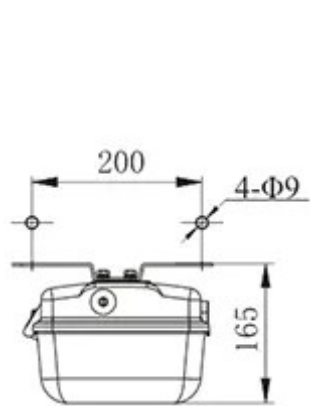
Ceiling type
